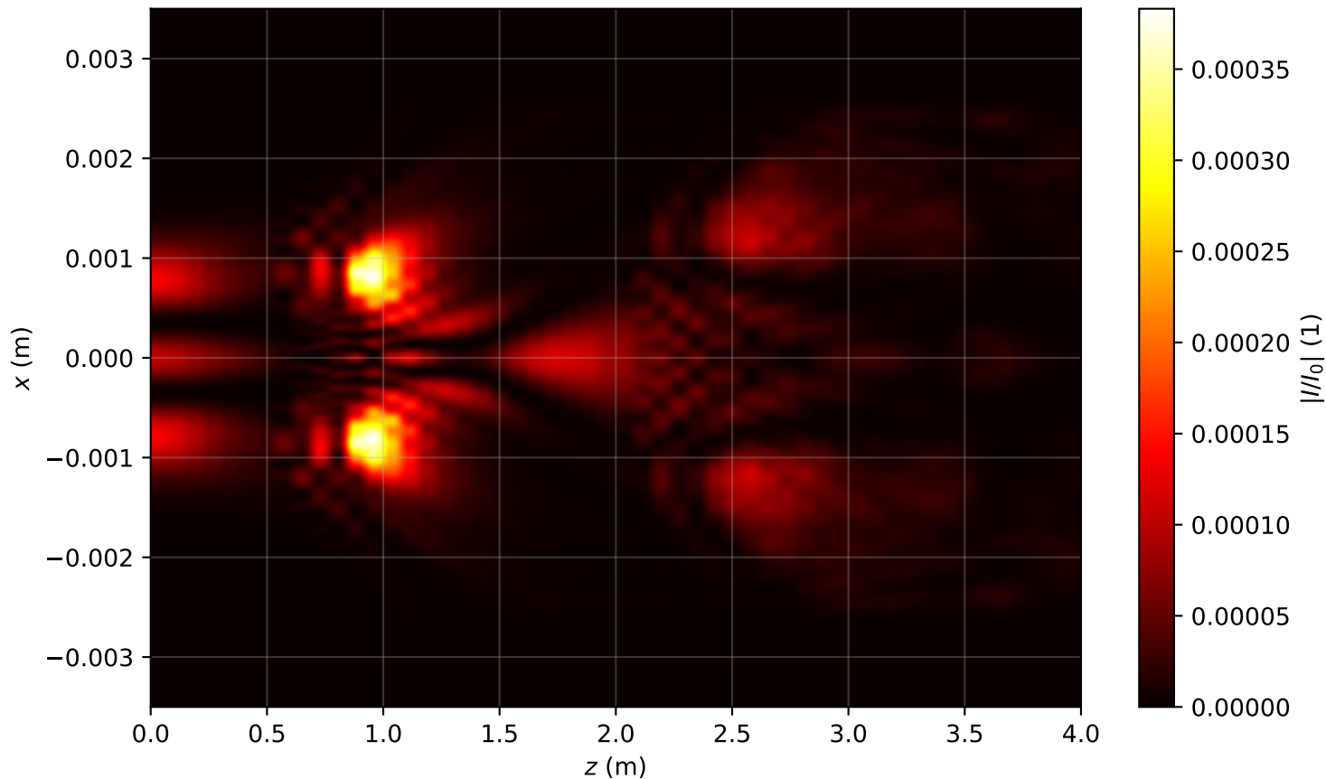
Intensity profile I(x, y = 0, z)/I_0 , P_{in}=9.0P_{cr} , artificial time
